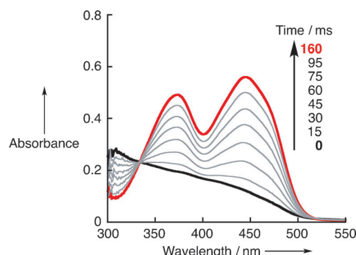
Figure 3. Changes in the UV/Vis absorption spectrum during the oxidation of \text{FMNH}_2 (50 \mu\text{M} ) by \text{O}_2 (0.68 mM) under an \text{O}_2 ( 5.0 \times 10^{-2} MPa)/ \text{N}_2 ( 5.0 \times 10^{-2} MPa) gas mixture in an aqueous phosphate buffer (pH 6.0) after mixing an \text{O}_2 -saturated buffer solution with a buffer solution of \text{FMNH}_2 under \text{N}_2 . \text{FMNH}_2 was formed in the reduction of FMN (100 \mu\text{M} ) by \text{H}_2 (bubbling for 10 min) with 1 (5.0 \mu\text{M} ) under normal pressure at 298 K.
